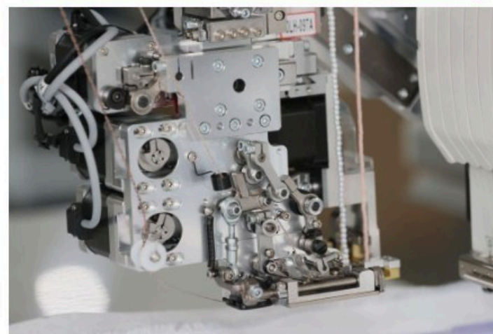
可加装各类装置让绣品更具价值 Possible To Add All Kinds Of Devices Make Your Design More Valuable
